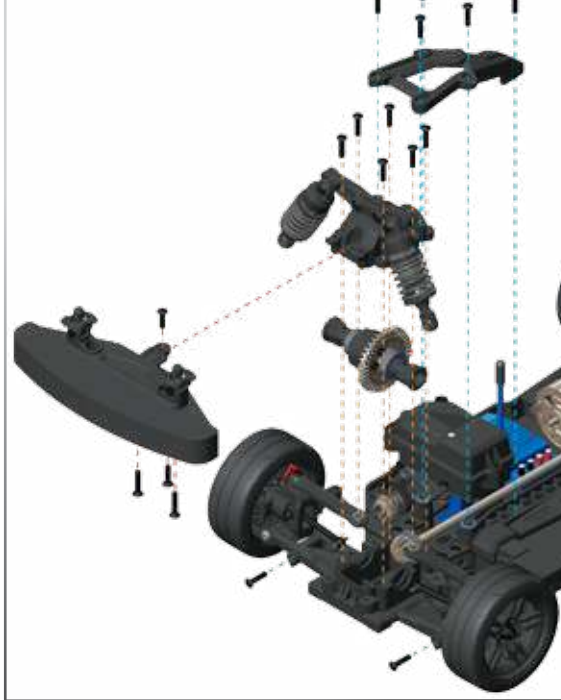
Front Differential Removal
