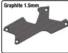
Graphite 1.5mm C-00180-276 Suspension arm stiffener - Rear - Right - Graphite 1.5mm - 1 pc
