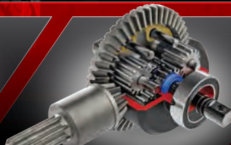
Steel-Gear Planetary Differentials
